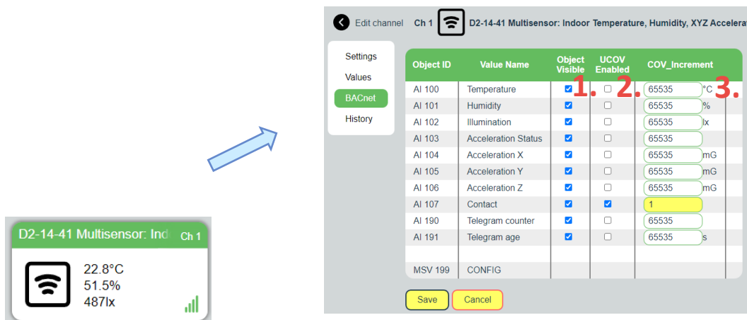
Fig. 6.8 Channel details – BACnet tab
