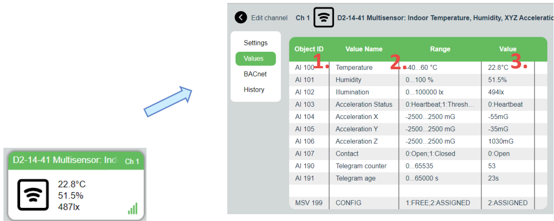
Fig. 6.7 Channel details – Values tab
