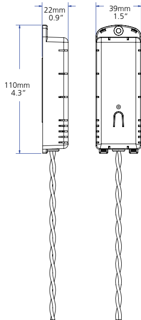
Leak Detector
