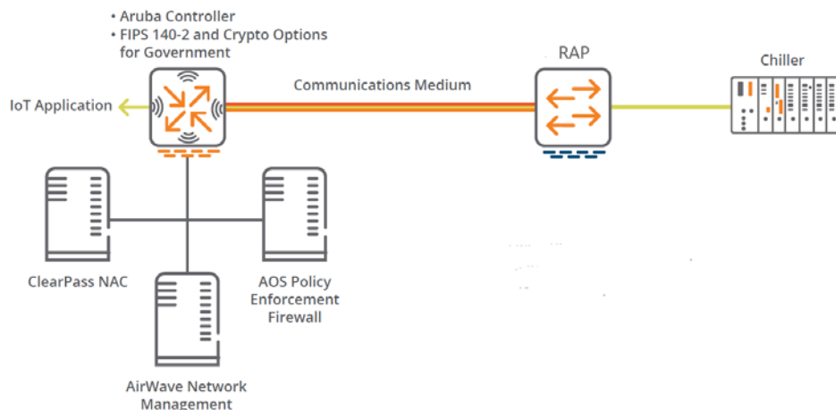
Remote Chiller Monitoring
