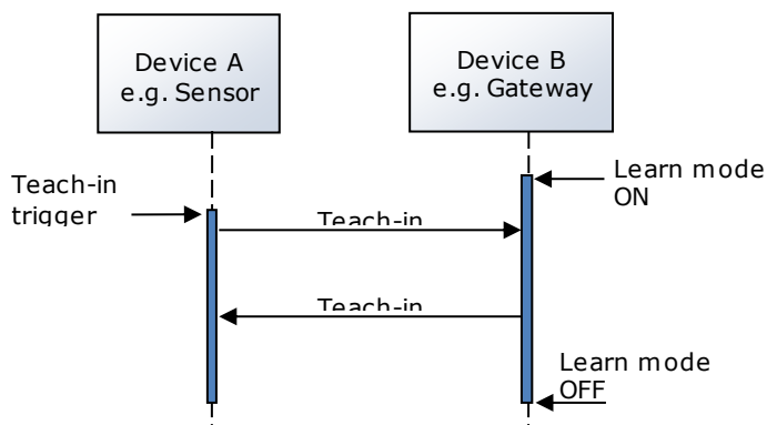
Figure 13. Schematic representation of the teach-in procedure
