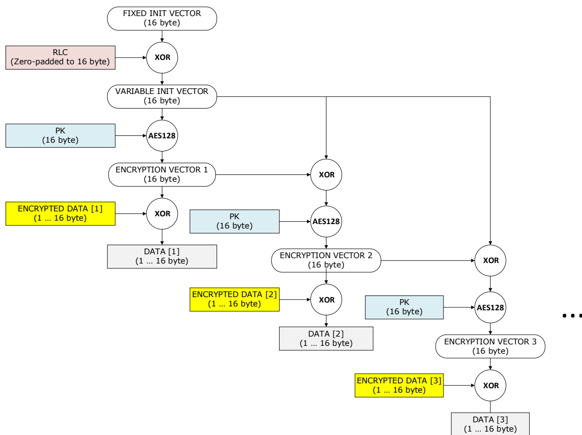
Figure 21. VAES-128 decryption process
