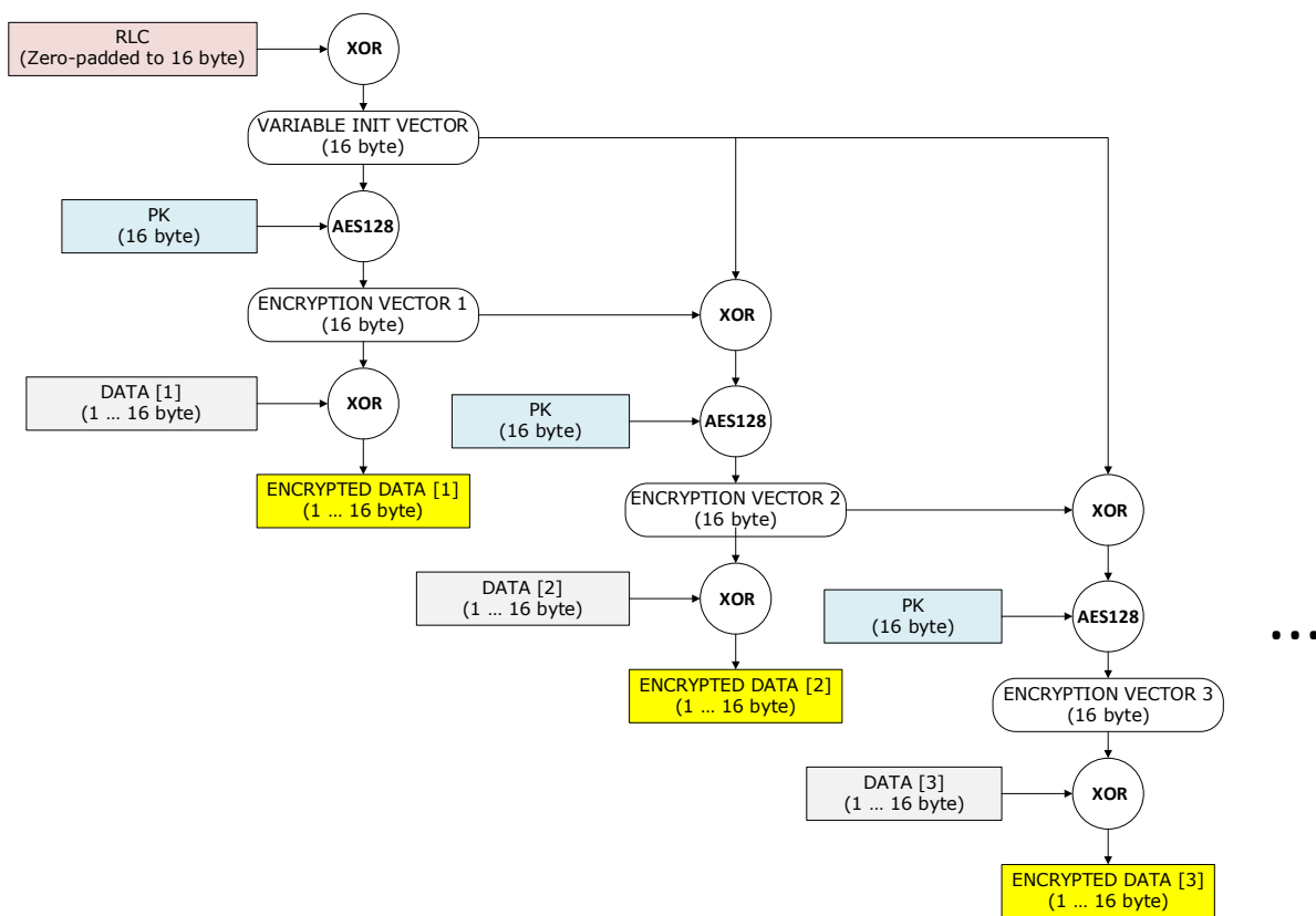
Figure 20. VAES-128 encryption process
