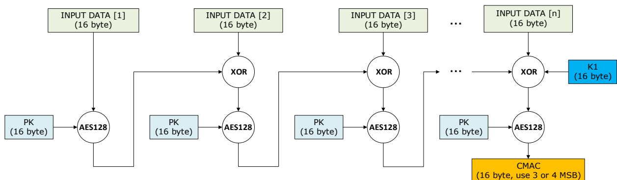
Figure 23. CMAC generation for input data with multiple of 16 bytes size
