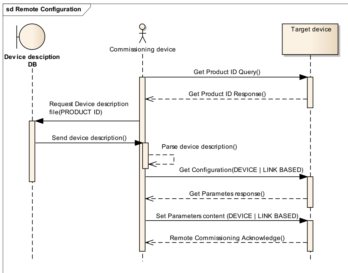
Figure 12 Remote configuration
