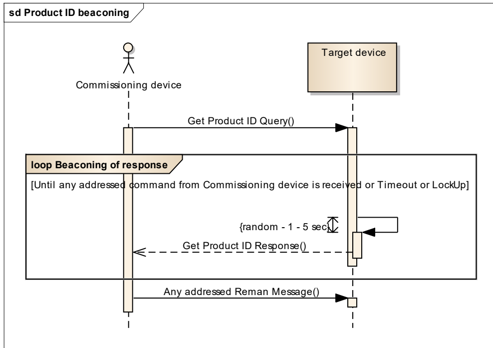
Figure 15 Product ID Beaconsing sequence
