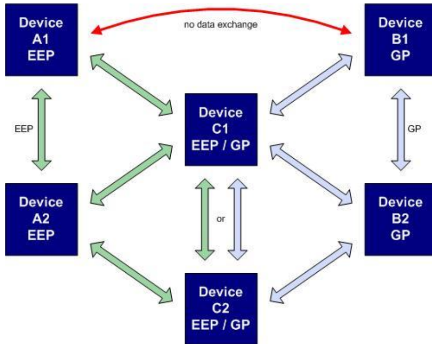
FIGURE 6.1: CONNECTION SCENARIOS
