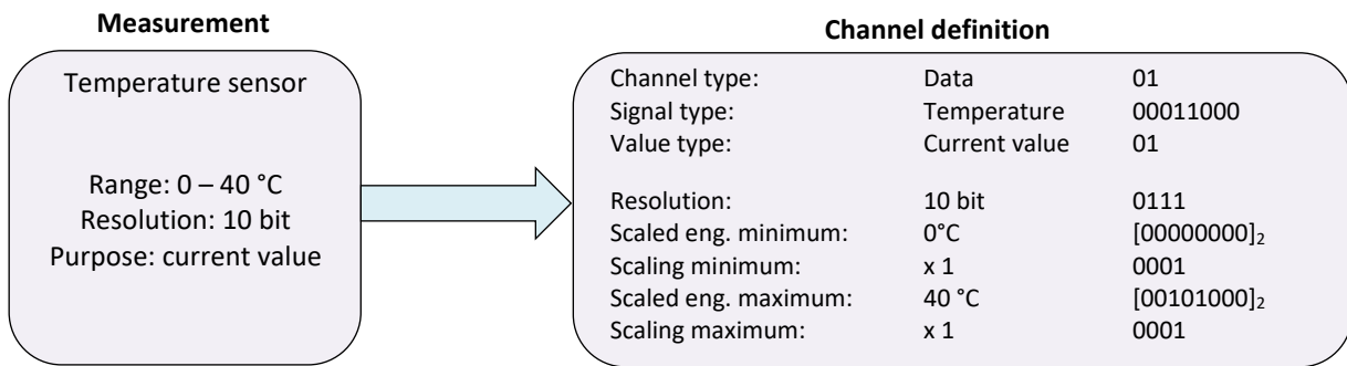
FIGURE 3.3: EXAMPLE TEMPERATURE SENSOR DEFINITION
