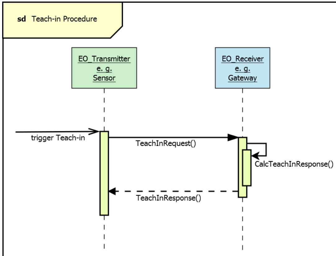
FIGURE 4.1: TEACH-IN PROCEDURE
