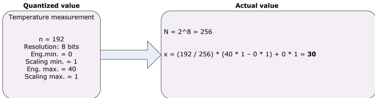
FIGURE 3.8: EXAMPLE RECALCULATION ACTUAL VALUE
